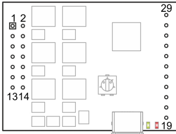
Figure 3-3 Pin Assignment
