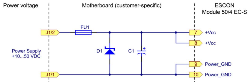
Figure 5-17 Wiring of Voltage Supply Cable
