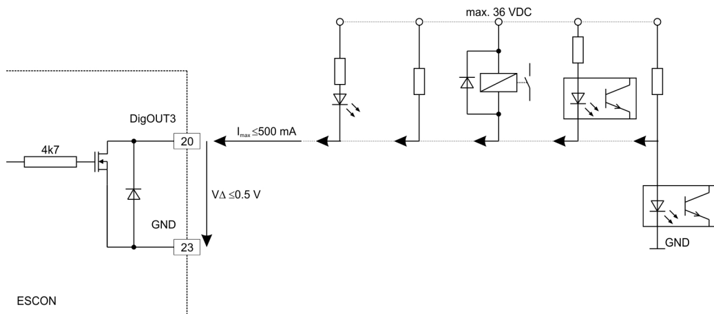
Figure 3-9 DigOUT3 Wiring Examples (analogously valid also for DigOUT4)
